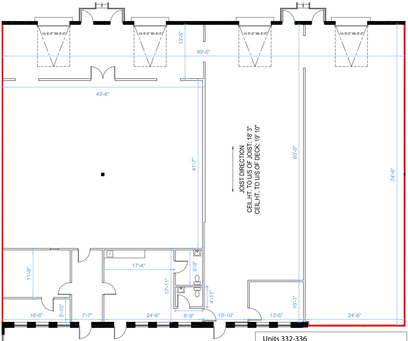
KEY PLAN
