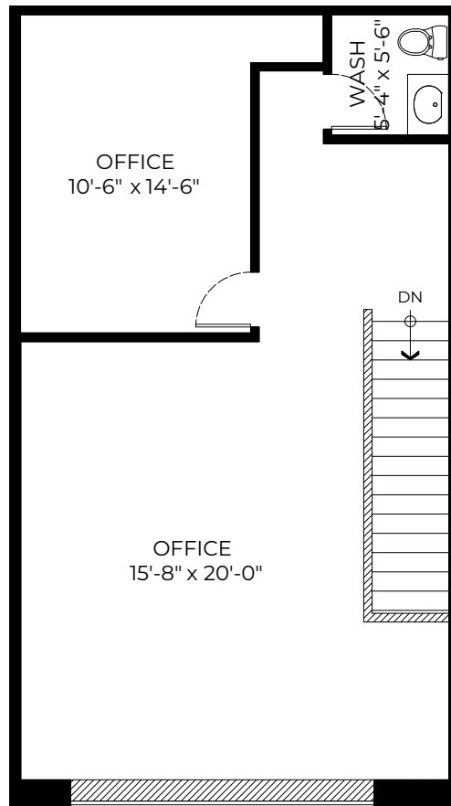
UPPER FLOOR PLAN Ceiling Height: 8'-0"
