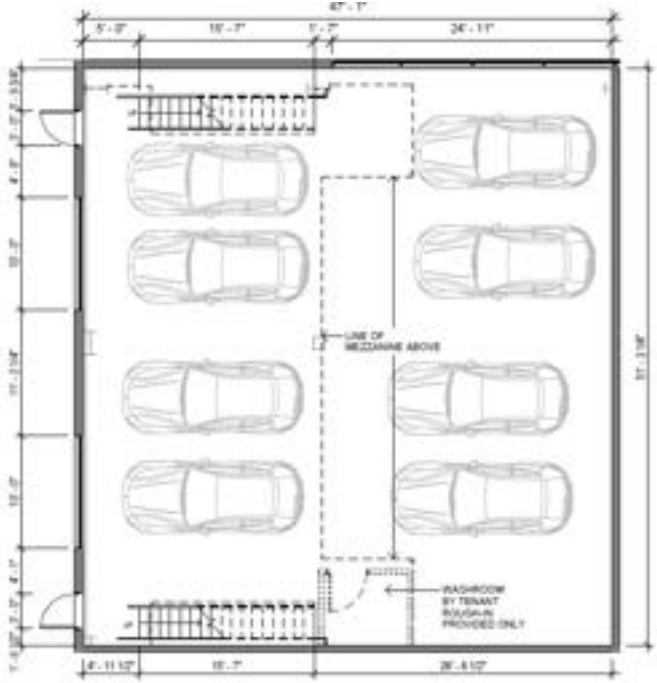
MAIN LEVEL
