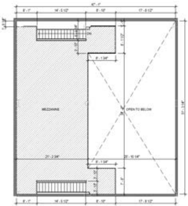
MEZZANINE LEVEL
