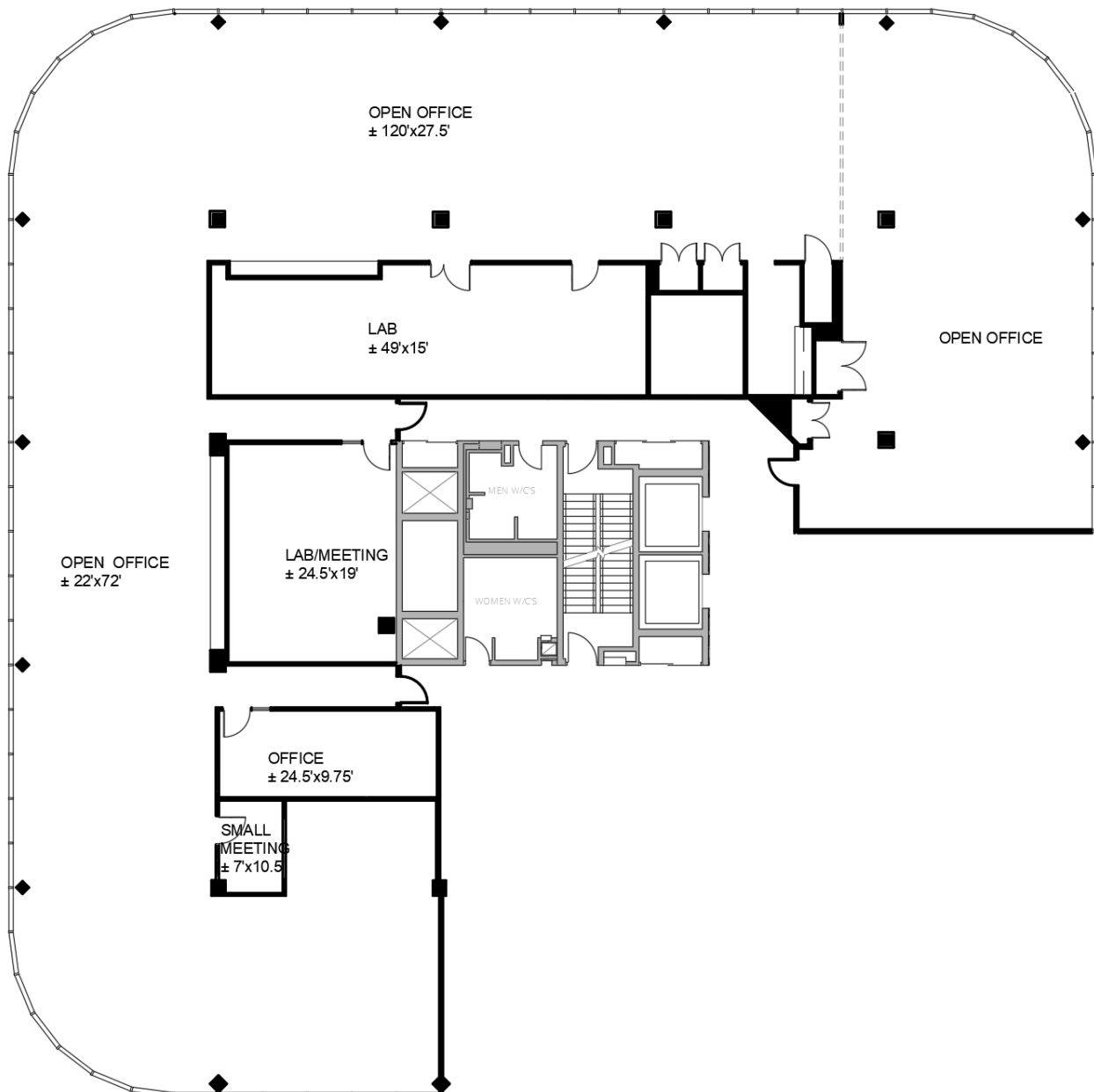
KEY PLAN
