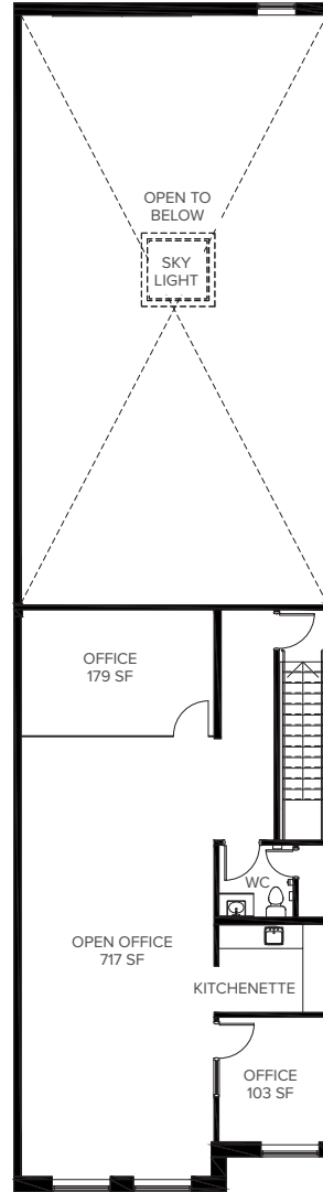
SECOND FLOOR
