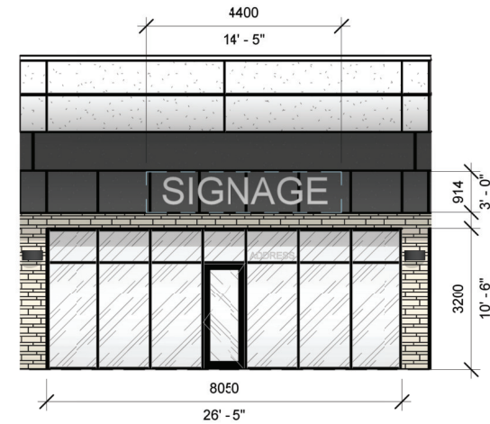
UNIT ELEVATION
