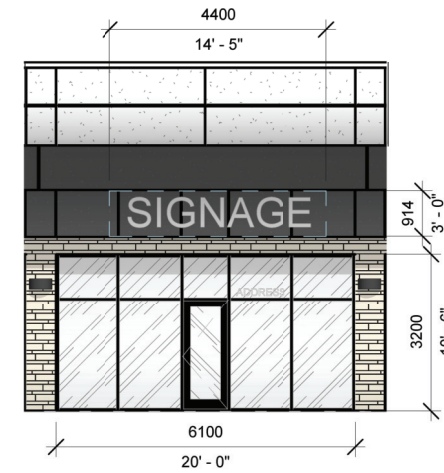
UNIT ELEVATION
