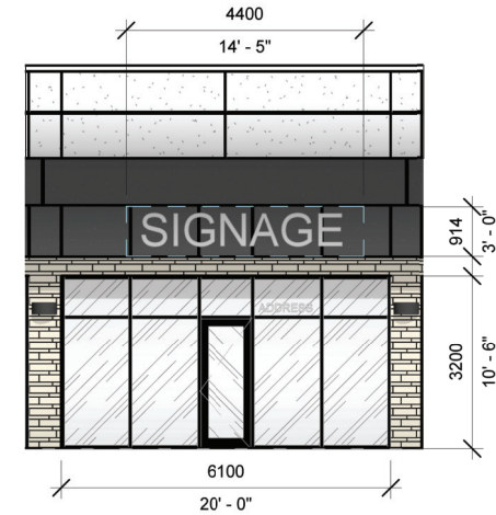
UNIT ELEVATION
