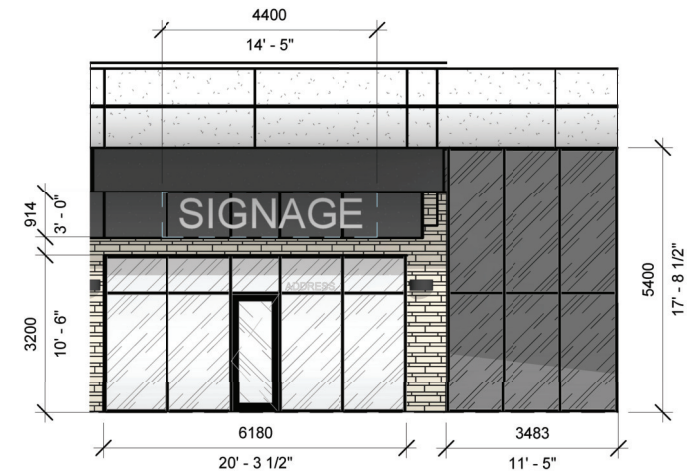
UNIT ELEVATION
