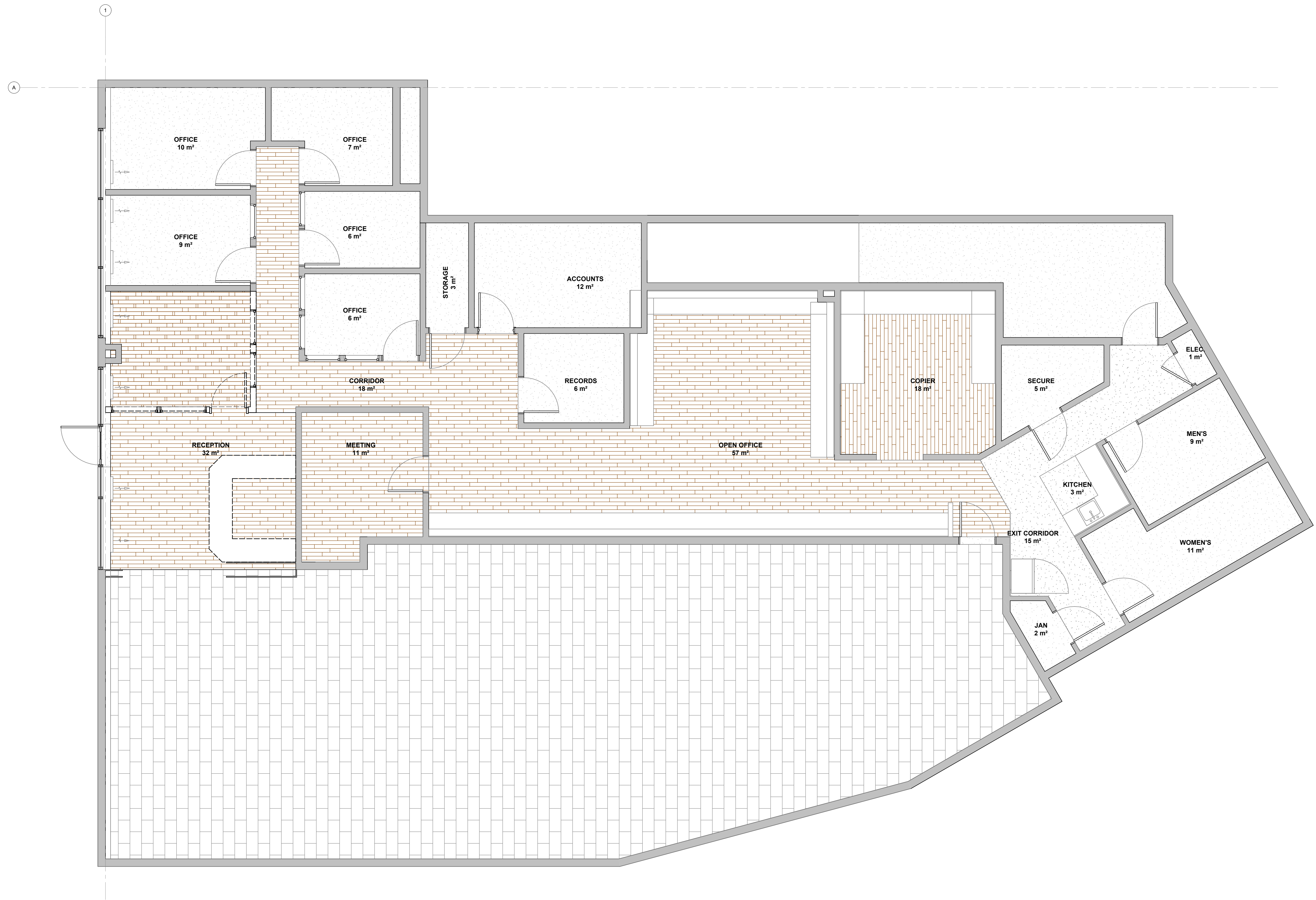
1 FLOOR PLAN - L1 NEW 1/4" = 1'-0"
