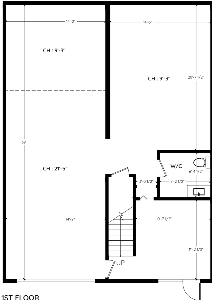
1ST FLOOR 1,199 SQ.FT. CH: 8'-0"
