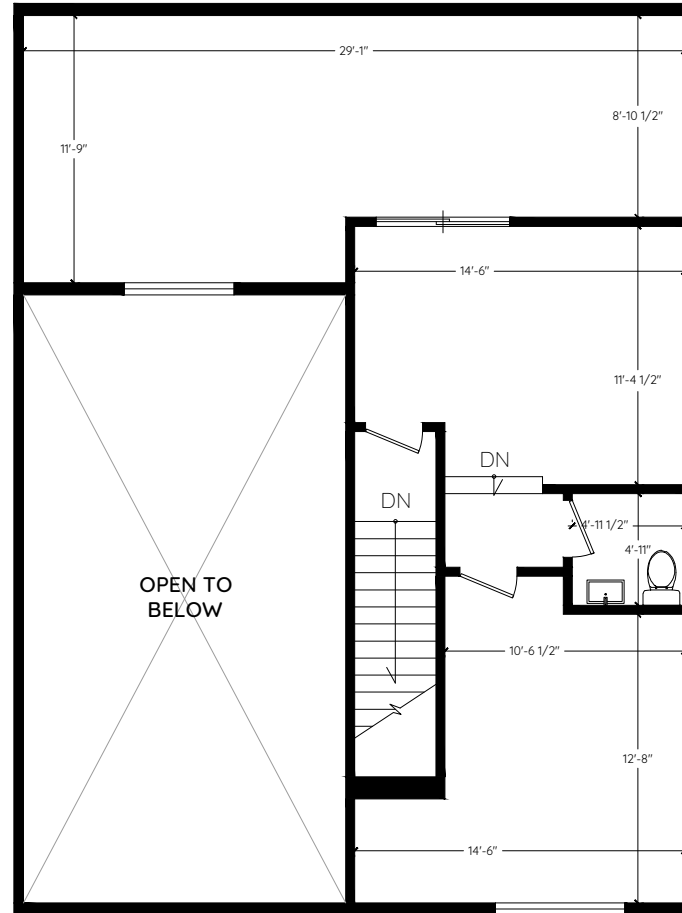
2ND FLOOR 801 SQ.FT. CH: 8'-1"
