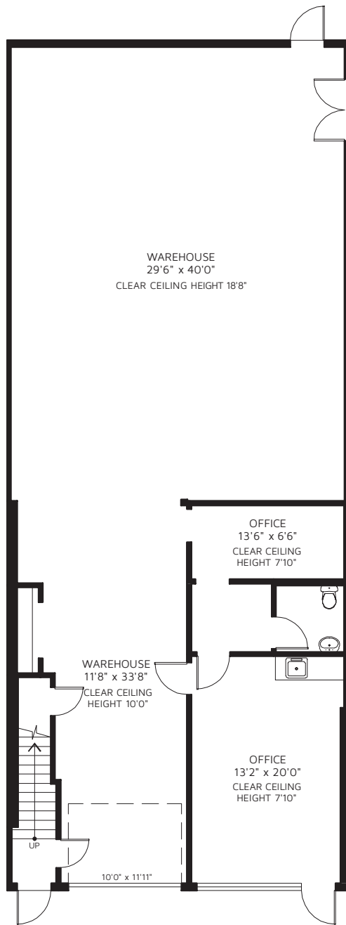
MAIN FLOOR
