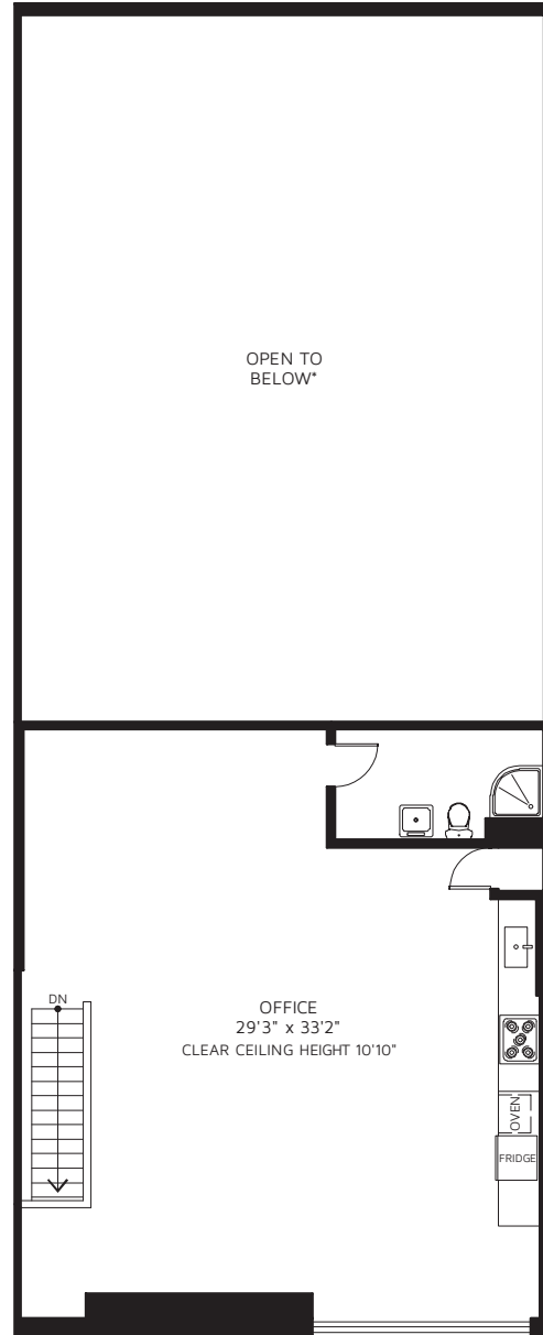
UPPER FLOOR
