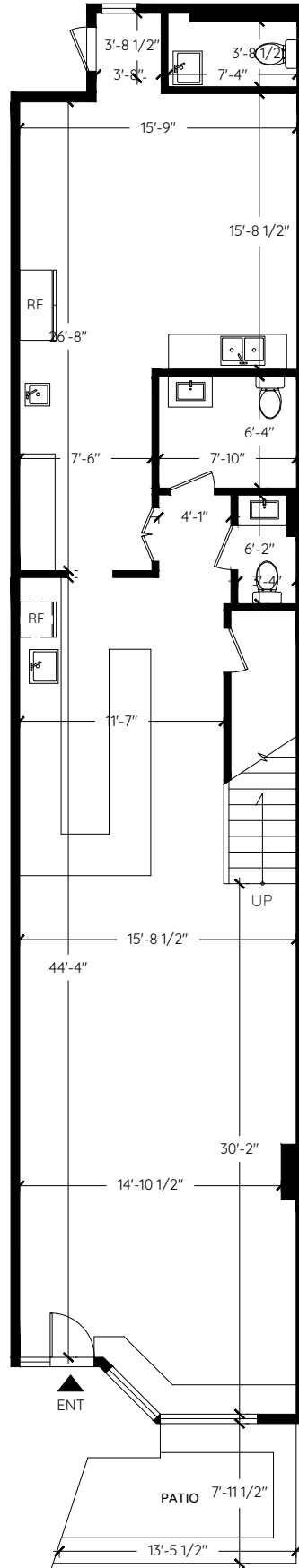
MAIN FLOOR 1,306 SQ.FT. CH: 21'-6"
