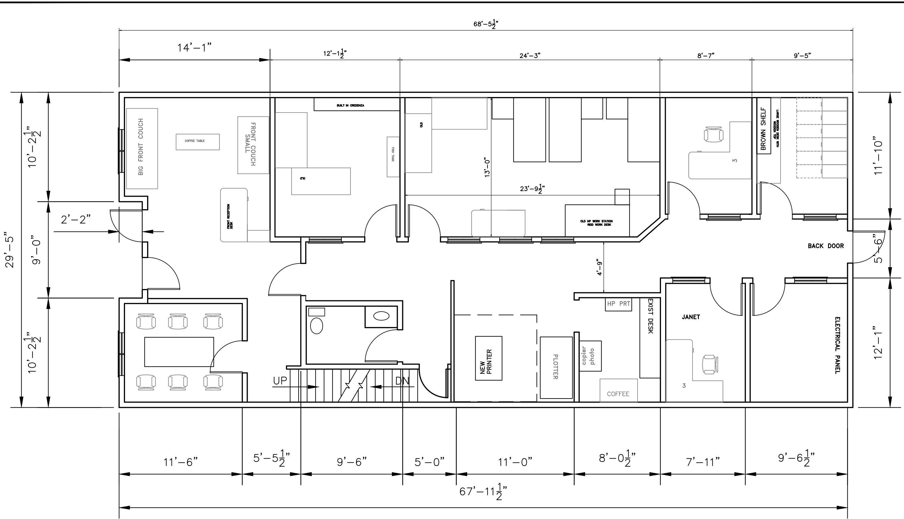
MAIN FLOOR PLAN 1994 SQ.FT
