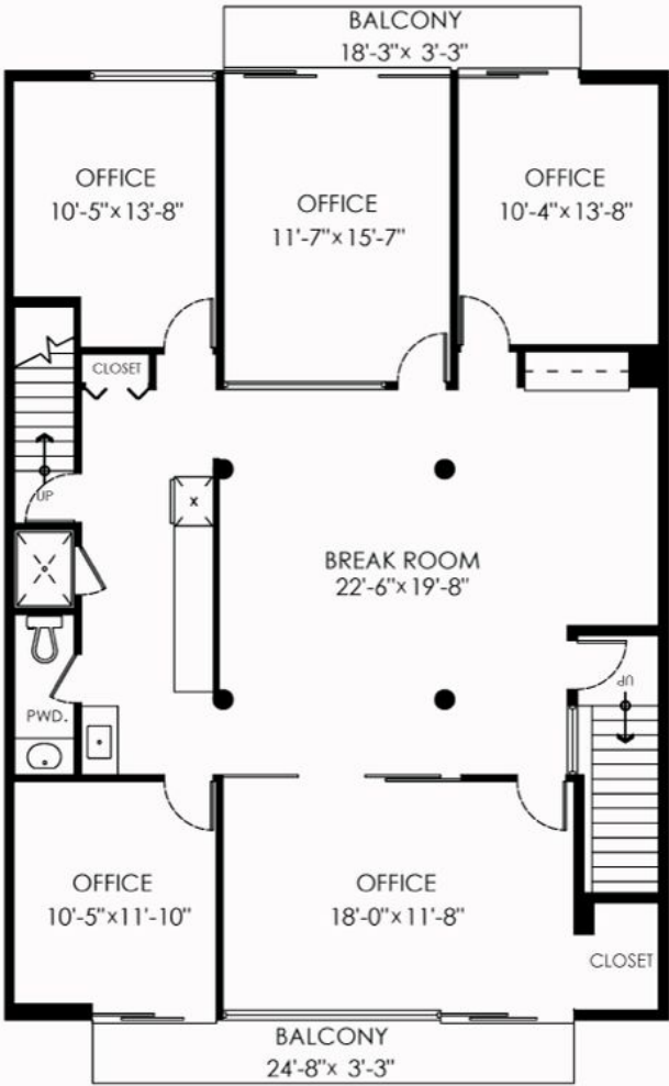
Top Floor Plan Floor Area: 1647 sq.ft. Ceiling Height: 8'-8"
