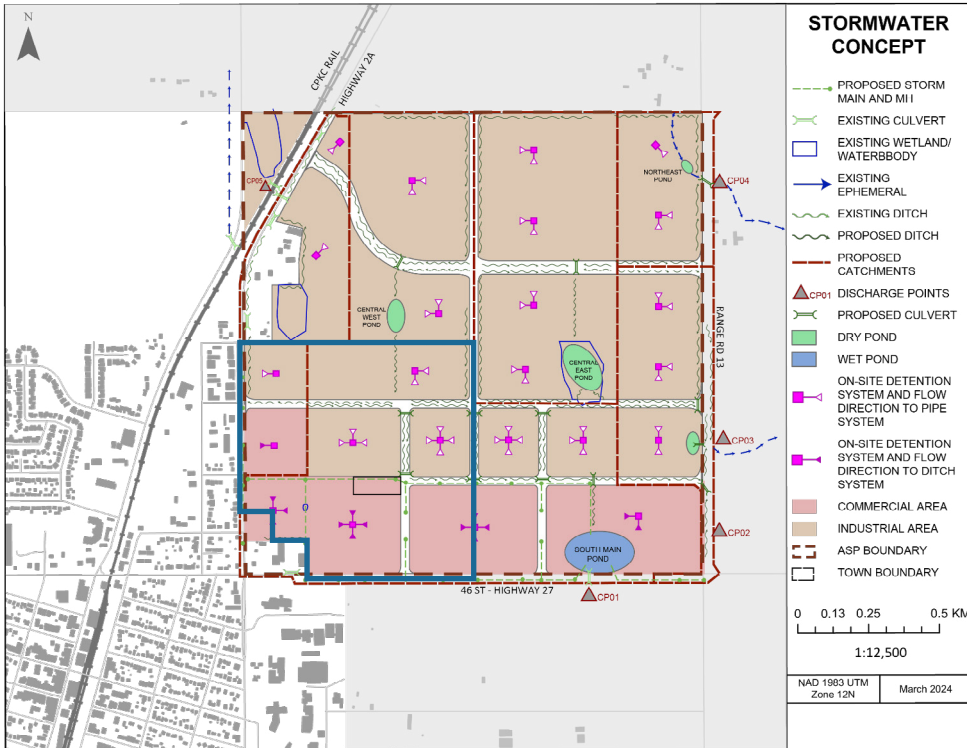
Figure 9: Stormwater Concept Map
