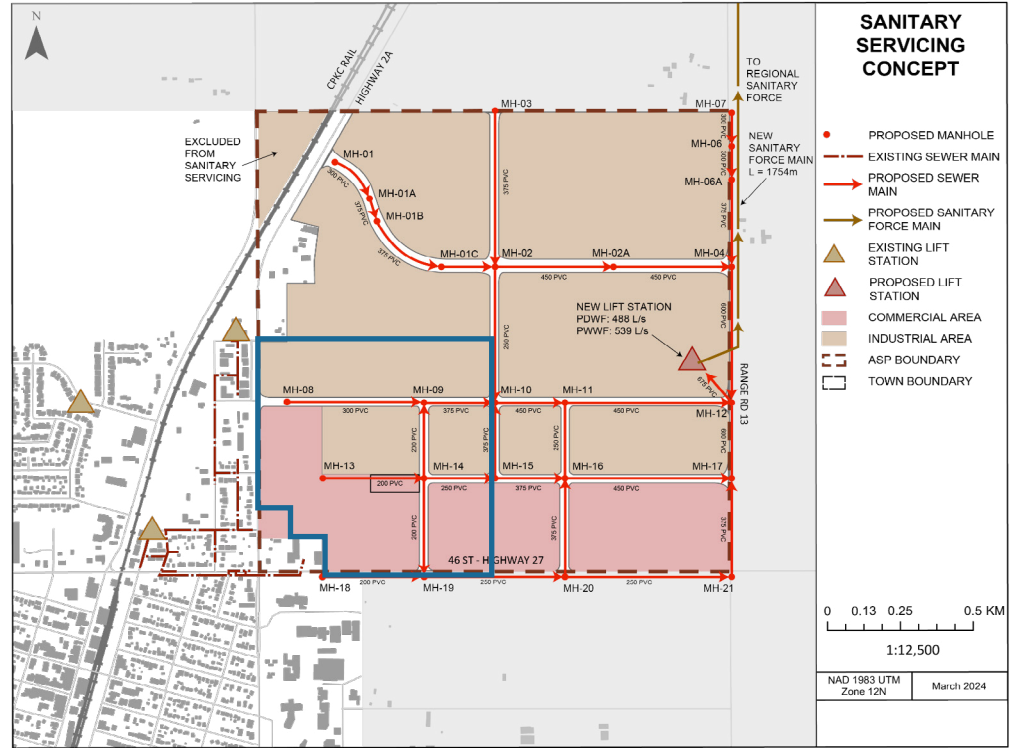
Figure 10: Sanitary Servicing Concept Map
