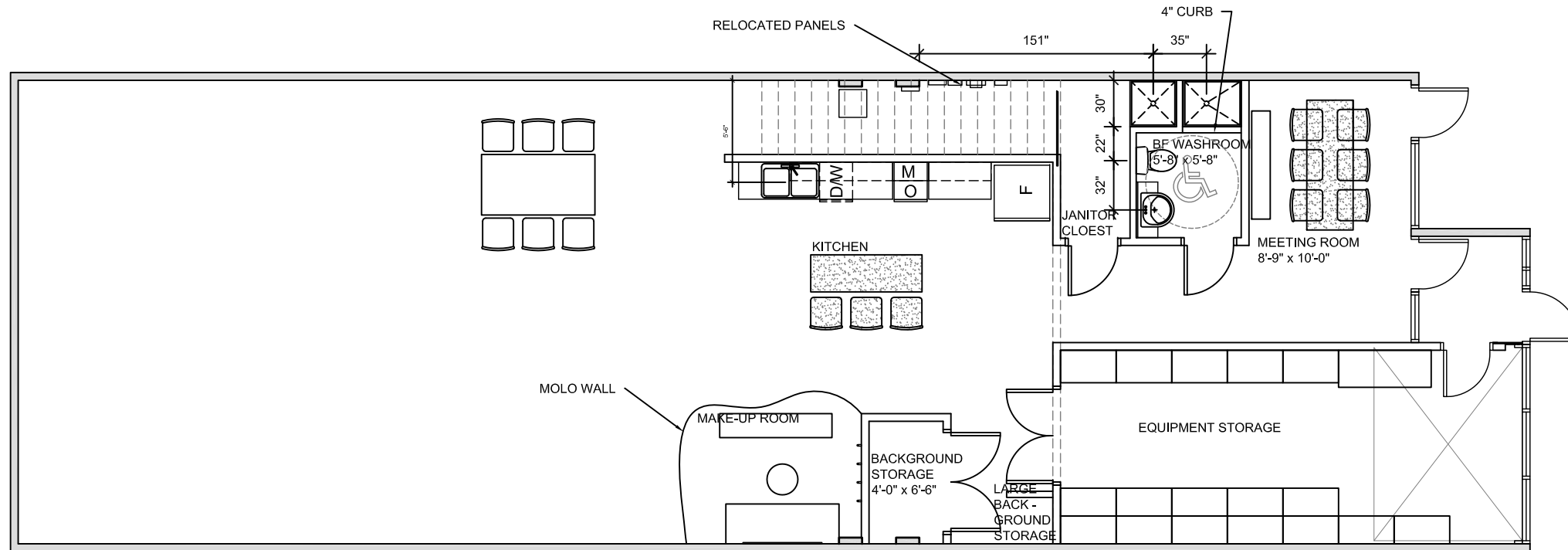
1 MAIN FLOOR SP-1 SCALE: 1/8"=1'-0"
