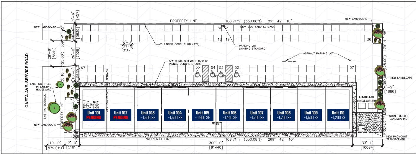
SITE PLAN / LANDSCAPE PLAN
