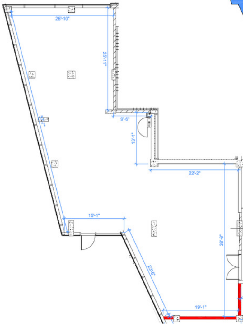
KEY PLAN
